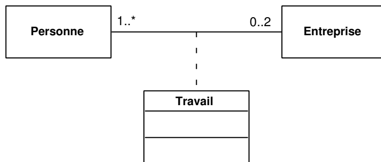
FIG. II. 28 – Diagramme de classes D_1
