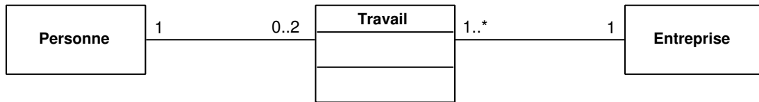
FIG. II. 29 – Diagramme de classes D_2
