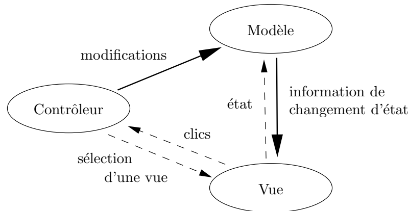
FIG. IV. 4 – Architecture MVC
