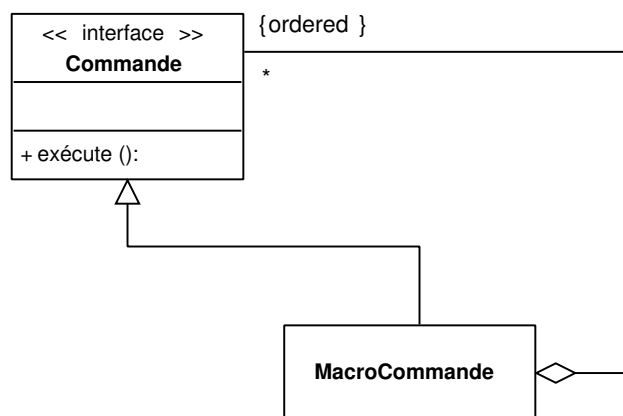
FIG. V. 8 – Macro commandes
