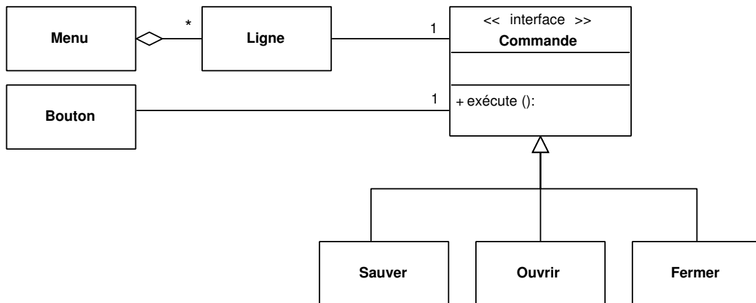
FIG. V. 7 – Patron Commande
