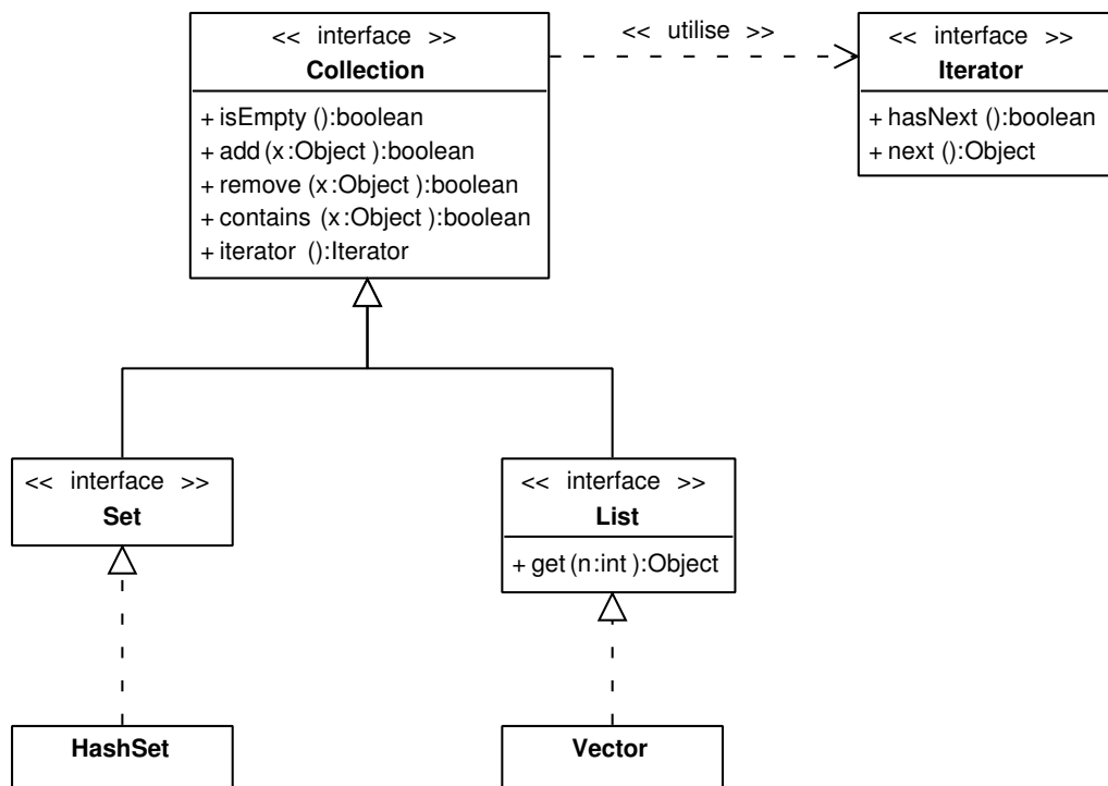
FIG. II. 49 – Les collections Java
